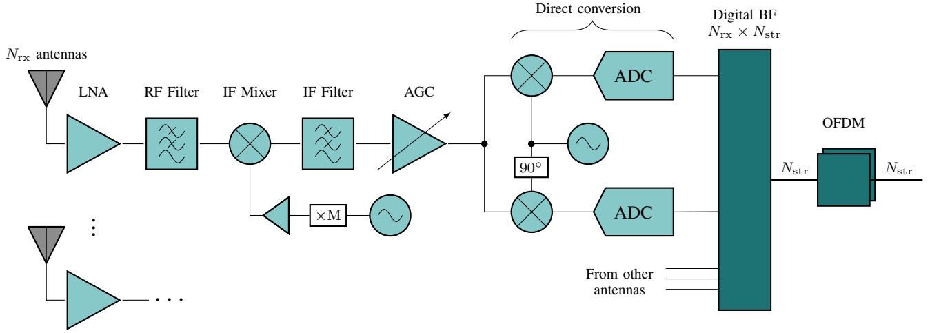
Fig. 3. High-level architecture of a fully-digital superheterodyne receiver architecture. The architecture supports N_{rx} antennas and N_{str} digital streams. The light green boxes represent analog and the dark-green boxes the digital components. In the RF front-end, some component are not shown.
