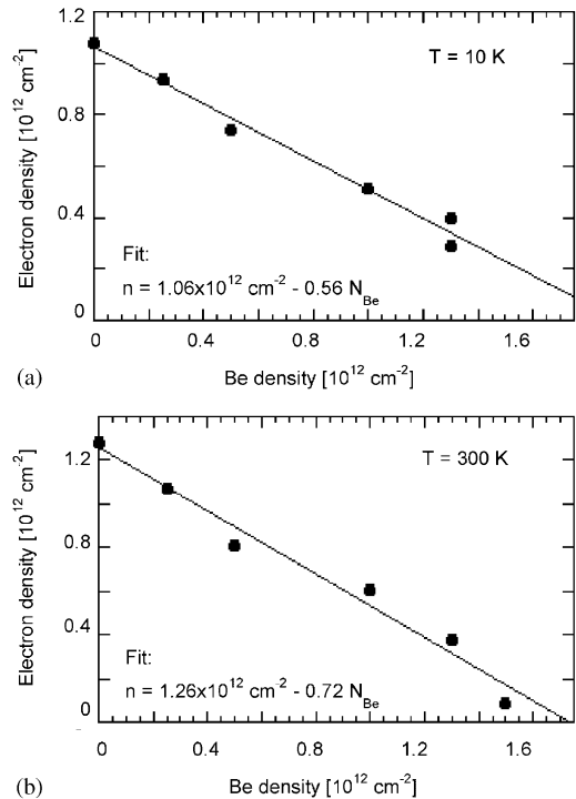
Fig. 3. Electron concentration as a function of Be doping at temperatures of 10 and 300 K. The data are fitted with linear functions.
