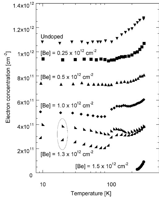
Fig. 1. Electron concentration for different temperatures and Be doping levels as determined by Hall measurements.
