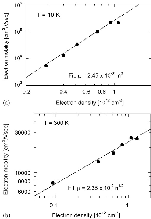
Fig. 4. Electron mobility as a function of electron density at temperatures of 10 and 300 K. The data are fitted with power laws.
