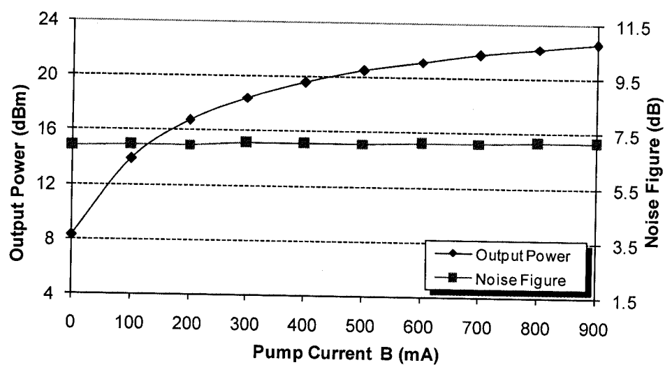
Figure 3. Output power and noise figure vs. pump current
