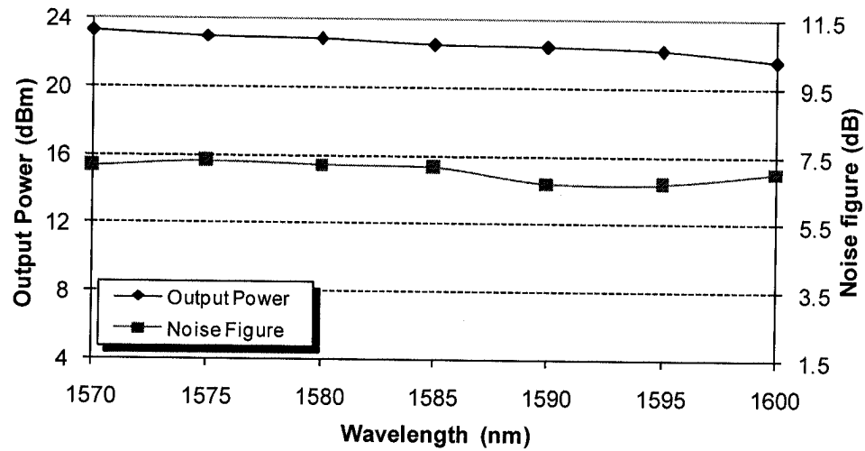
Figure 4. Output power and noise figure vs. wavelength
