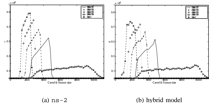
Fig. 10. Probability density functions for the congestion window and queue size for the Y-shape topology with 4 TCP flows and 10% background traffic (500Mbps bottleneck).
