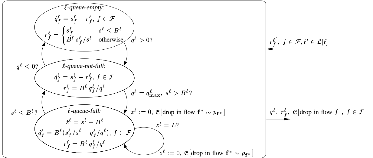
Fig. 3. Hybrid model for the queue at link \ell . In this figure, q^\ell is given by (2), the s_f^\ell, f \in \mathcal{F} are given by (3), and s^\ell := \sum_{f \in \mathcal{F}} s_f^\ell, \forall \ell \in \mathcal{L} .
