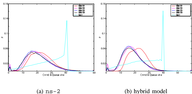
Fig. 9. Probability density functions for the congestion window and queue size for the Y-shape topology with 4 TCP flows and 10% background traffic.
