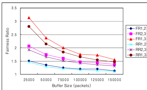
Fig. 15. Average throughput fairness between the three different TCP-Sack flow sets simulated on the Abilene Network
