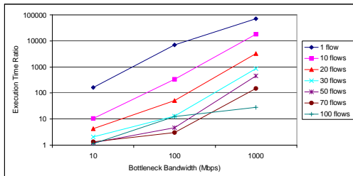
Fig. 12. Execution time speedup of hybrid model over ns-2 simulation for dumbbell topology with 100 ms propagation delay bottleneck.
