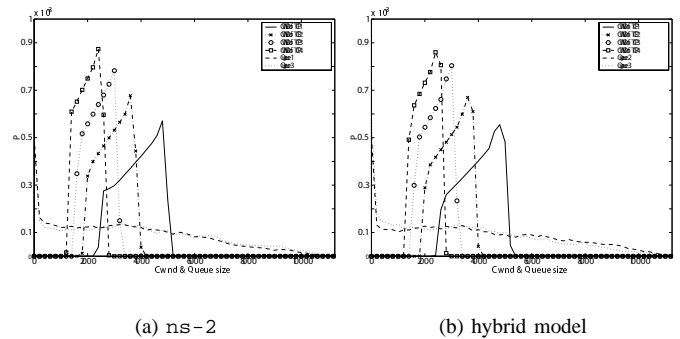
Fig. 11. Probability density functions for the congestion window and queue size for the parking-lot topology (500Mbps bottleneck) with 4 TCP flows and 10% background traffic. These were computed from simulations using ns-2 (left) and a hybrid model (right).
