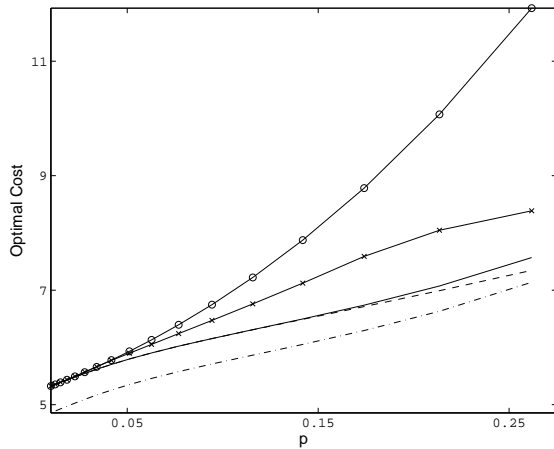
Fig. 3. Optimal costs ( \lambda = 2.2 ) as a function of the drop probability for: policy v(k) \equiv 1 (o); optimal policy with v \in \{1, 2\} (solid); optimal policy with v \in \{1, 2, 3\} (dashed); optimal policy with v \in \{0, 1, 2\} (dash-dotted); simplified optimal policy with v \in \{1, 2, 3\} and T = 5 (cross).
