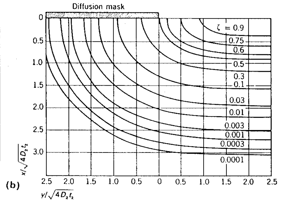
Diffusion contours at the edge of an oxide window for (a) constant source diffusion (pre-deposition), and (b) limited source diffusion (drive-in).
