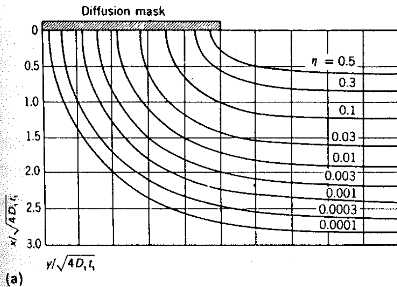
Diffusion contours at the edge of an oxide window for (a) constant source diffusion (pre-deposition), and (b) limited source diffusion (drive-in).
