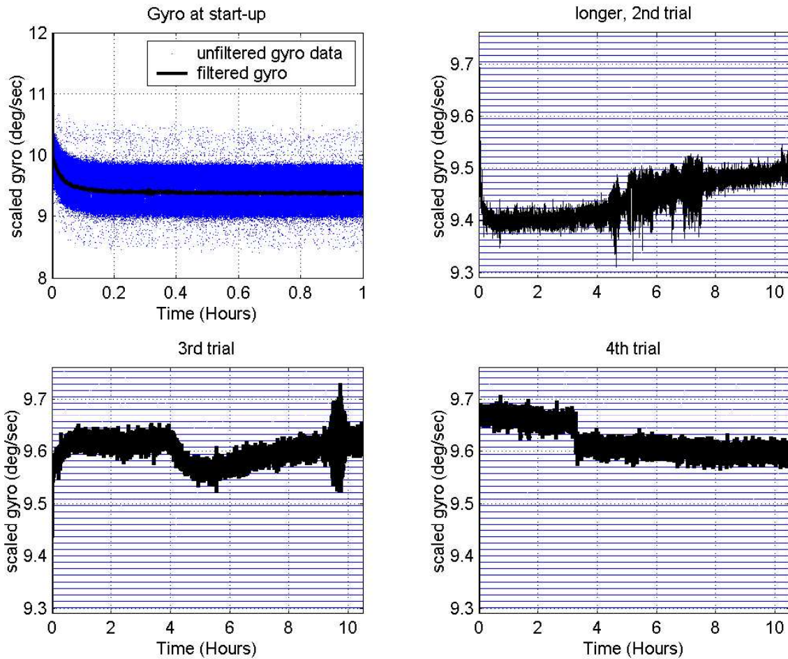
Figure 6-16: Drift of gyro DC bias (offset) over time. These data were taken with the gyro at rest and the ambient temperature steady to within a few degrees Fahrenheit (in our air conditioned laboratory). Temperature has a significant effect on bias. The upper left plot here shows the change in bias typical for the device as it warms up after power is initially sent to it.
