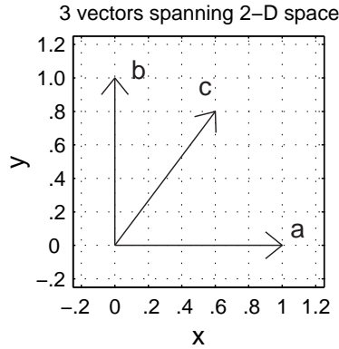
Figure 6-2: A 3-sensor array spanning 2-D space. The three vectors shown point in the directions \mathbf{a}=[1\ 0] , \mathbf{b}=[0\ 1] , and \mathbf{c}=[.6\ .8] . Sensors aligned along these vectors form a sufficient set for fault detection, since the three vectors form a linearly dependent set. Specifically, \mathbf{c} = .6\mathbf{a} + .8\mathbf{b} .
