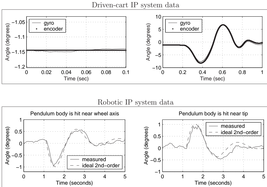
Figure 5-5: Disturbance rejection of the IP cart system. At right, top is the transient response of the pendulum to a disturbance applied at its tip. The controller for the cart system used the gyro (and accelerometer) to estimate pendulum angle and angular velocity when these data were taken. The figure at left, top plots a subset of the same data in the period just before the disturbance is applied, to examine the gyro and encoder measurements of pendulum angle as the pendulum balances in steady state. As in Figure 5-4, the 90 Hz resonance seen in Figures 5-3 is not in evidence here. Each encoder count corresponds to an angle of 0.09^\circ , as illustrated in the encoder data shown in Figure 5-4, and the gyro data indicate angular deflections on the order of 0.01^\circ - 0.02^\circ during this time. Thus, it is not surprising the encoder registers a constant value here while the gyro does not.) The lower two data sets show the transient response of the DIPR robot described in Chapter 7 for comparison. (See the text for more detail.) The data shown in the lower plots also appears in Figure 1-15 on page 1-15 of Chapter 1.
