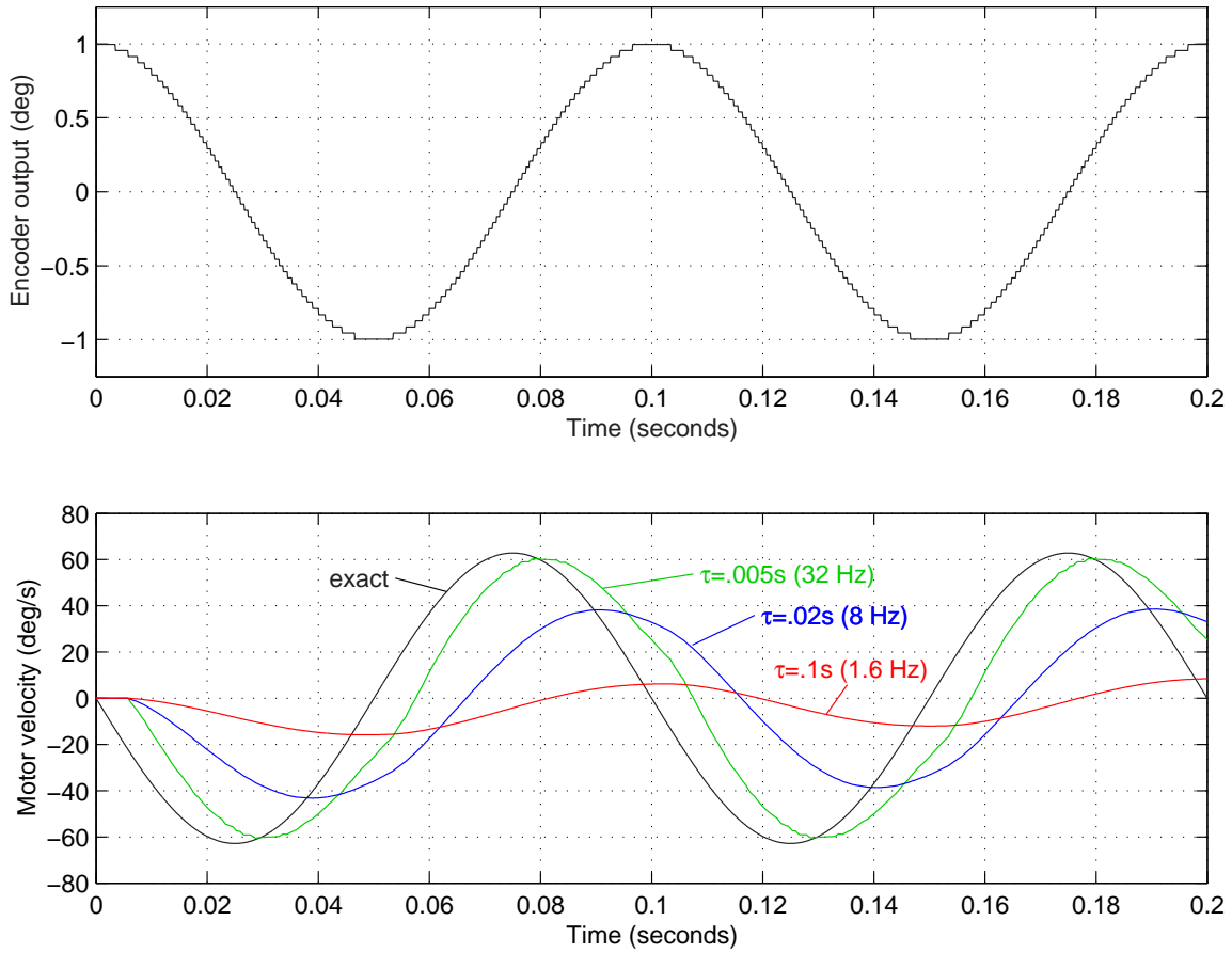
Figure 7-12: Theoretical filtering of time-based velocity estimate. This plot is intentionally formatted to facilitate direct comparison with Figure 7-9 on page 334. The data present simulations of the "time-based" velocity estimation method described in detail in the text, which uses the time interval between encoder counts to estimate the relative velocity between each wheel and the robot chassis. The particular estimation algorithm used to produce the plots above compares any current zero-order-hold estimate with an upper bound on the magnitude of the velocity. This upper bound is a velocity one would obtain by dividing the smallest encoder increment by the time which has so far elapsed since the the previous change in encoder output was measured. This is a conservative adjustment to the estimate and provides what I refer to as "extra smoothing" in the resulting velocity signal. The three estimates on the lower plot use first-order low-pass filtering (corresponding to the labelled values of \tau ).
