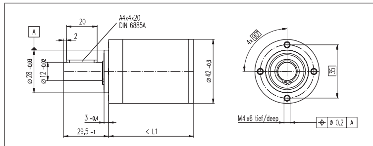
Figure F-2: Maxon GP 42 C planetary gearhead CAD drawing. (pt# 203114) Data below are reprinted from page 195 of the 2001 Maxon product catalog [129].
