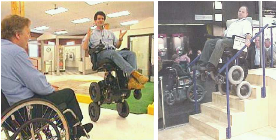
Figure 2-2: The iBOT in action. Image of Dean Kamen (at left) obtained from MSN Dateline website [142]. Image of person climbing stairs at a tradeshow taken from John Williamson's personal website [215].
