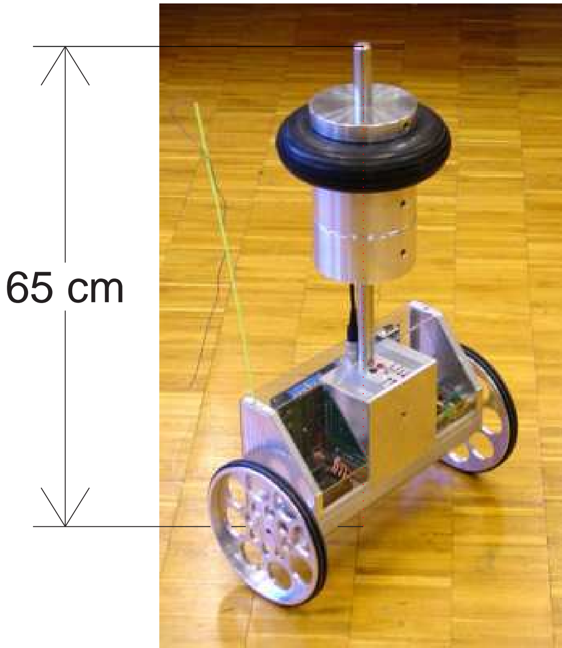
Figure 2-9: “JOE” inverted pendulum robot. Image obtained from “Joe: a Mobile, Inverted Pendulum”, by Felix Grasser and Aldo D’Arrigo and Silvio Colombi and Alfred Rufner [75].
