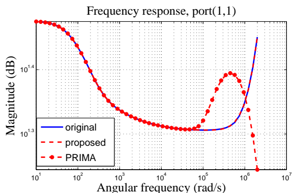
Fig. 3. MOR results for the original singular RLC model that contains a polynomial part. The response from the proposed approach is basically overlapping with the original one in the entire frequency band.
