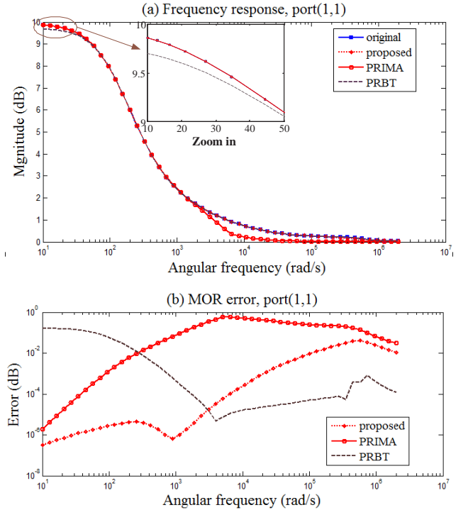
Fig. 1. Accuracy comparison of various MOR schemes for the indefinite strictly proper H_{sp}(s) . (a) The frequency response of port (1,1); (b) the numerical errors of the ROMs obtained by different algorithms. We can see that PRBT is not accurate in the low-frequency band, and PRIMA is inaccurate in the high-frequency band, but the proposed MOR result is indistinguishable with the original one in the whole frequency band.
