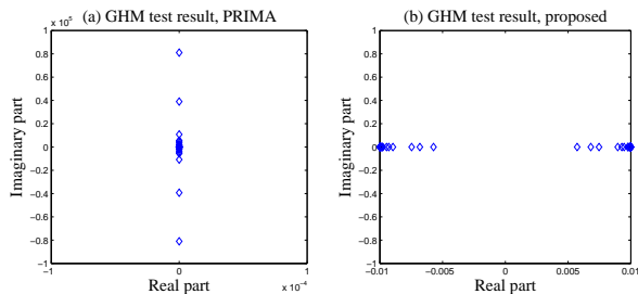
Fig. 2. (a) Passivity test results for the ROM by PRIMA (nonpassive); (b) test results for the ROM from the proposed MOR (passive).
